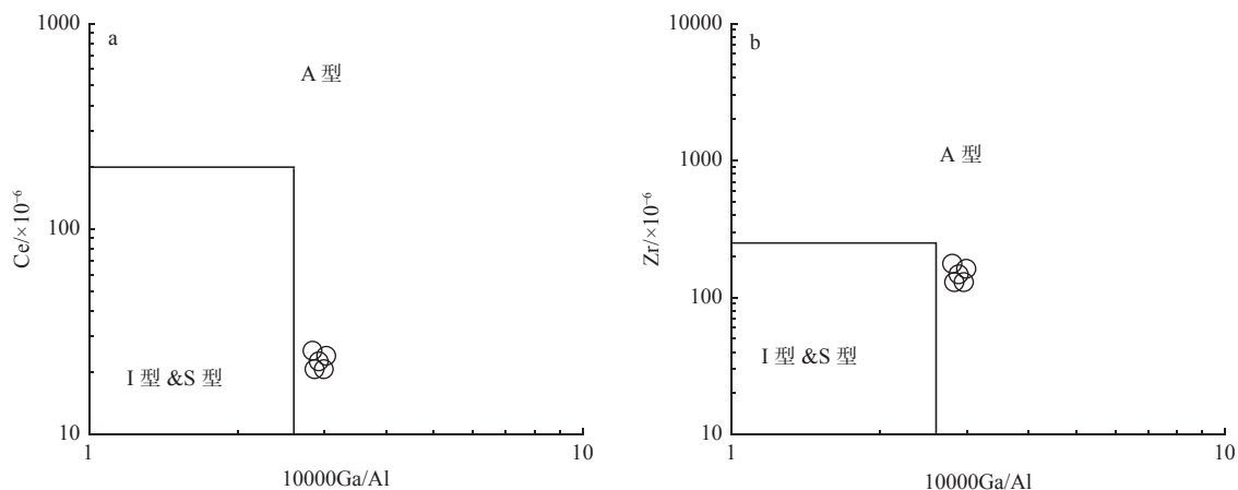
图 10 A 型花岗岩判别图解 (Whalen et al., 1987)
