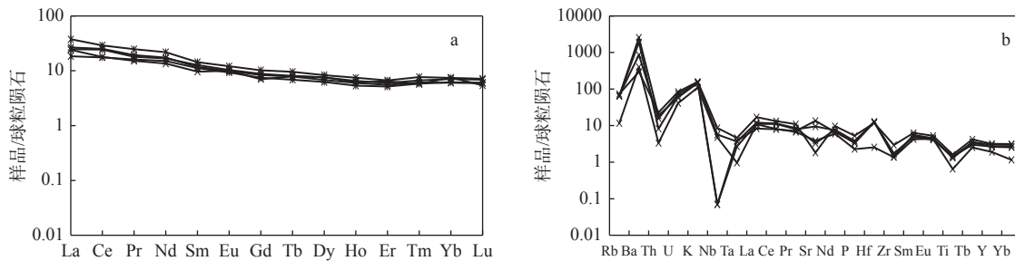
a—稀土元素蛛网图(球粒陨石值引自 Sun and McDonough, 1989); b—微量元素配分图
