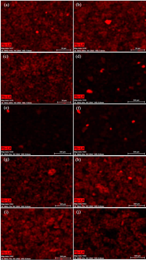
(a) ~ (c) the original sample of soil; (d) ~ (f) the heavy parts after washing; (g) ~ (i) the second heavy parts after washing; (j) the light parts after washing 图 3 土壤样品 EDS 面扫描能谱图
