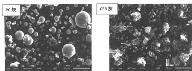
图 2 PC 灰和 CFB 灰的 SEM 图片 Fig. 2 SEM of of PC ash and CFB ash
