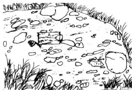
图4 四集庄东娘娘壕剖面熔岩胶结变质砾岩露头 Fig. 4 Picture showing an outcrop of the metamorphic conglomerate cemented by the lava, taken from the east of Sijizhuang village
