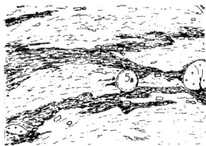
图5 含长石斑晶,具不同深浅条带片理化的中基性火山熔岩及其中花岗质砾岩(图4中A放大) Fig. 5 Magnification of the plate A in Fig. 4, in this figure a round with letter of "5角" is a coin and another with crosses is granite pebble
