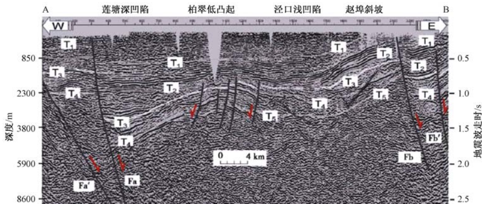
Fig. 2 Tectonic divisions of the Poyang Lake Basin
