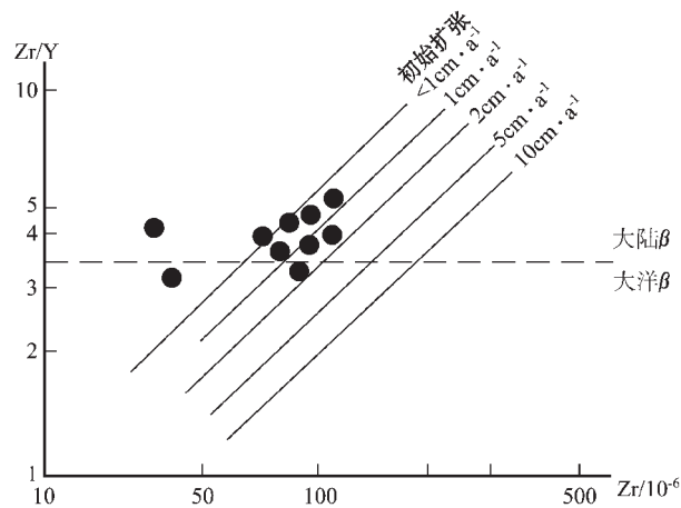
图5 库地蛇绿岩中玄武岩 Zr/Y-Zr 判别图 Fig. 5 Zr/Y-Zr discriminant diagram of basalt in the Küda ophiolite
