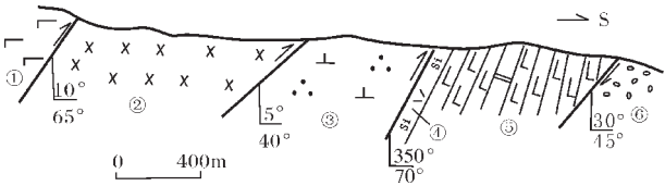
图2 北带蛇绿混杂岩路线地质剖面 Fig.2 Geological section of ophiolitic mélangé in the north belt
