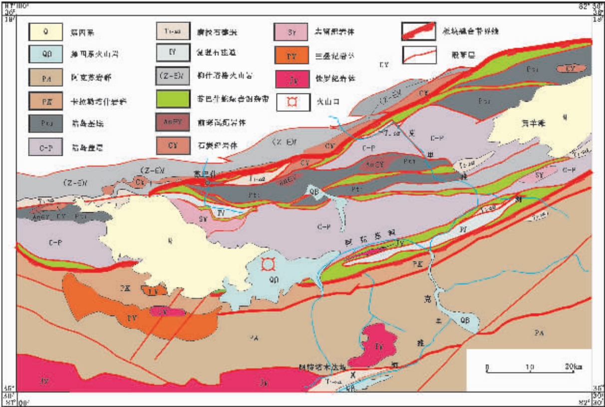
图1 于田县苏巴什—阿什库勒一带地质简图 Fig.1 Geological sketch map of Subexi-Ashikule, Yutian County
