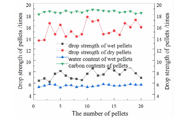
图 5 球团落下强度、含水率及碳含量 Fig. 5 Drop strength, water content and carbon content of pellet
