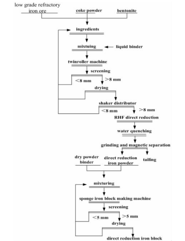
图 3 转底炉中试处理低品位难选矿 Fig. 3 Flowsheet of low grade refractory iron ore treated by the pilot test of rotary hearth furnace
