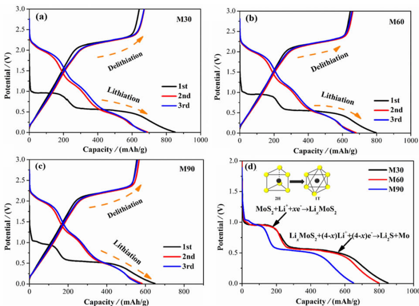
图 5 天然辉钼矿前三圈充放电曲线图(a) M30、(b) M60、(c) M90 和(d)首圈放电性能对比 Fig. 5 Charge - discharge curves of natural molybdenite in the first three cycles (a) M30, (b) M60, (c) M90, and (d) discharge performance comparison in the first cycle
